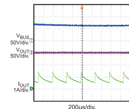
Short Steady State LED1 + to GND
