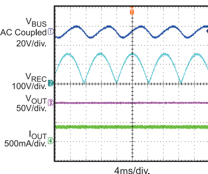
Short Steady State LED1 + to LED1 -
