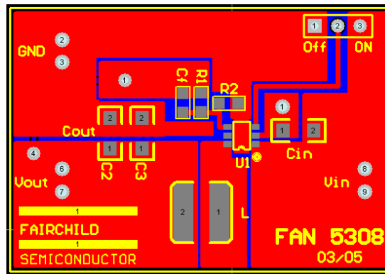
Figure 17. Recommended PCB Layout
