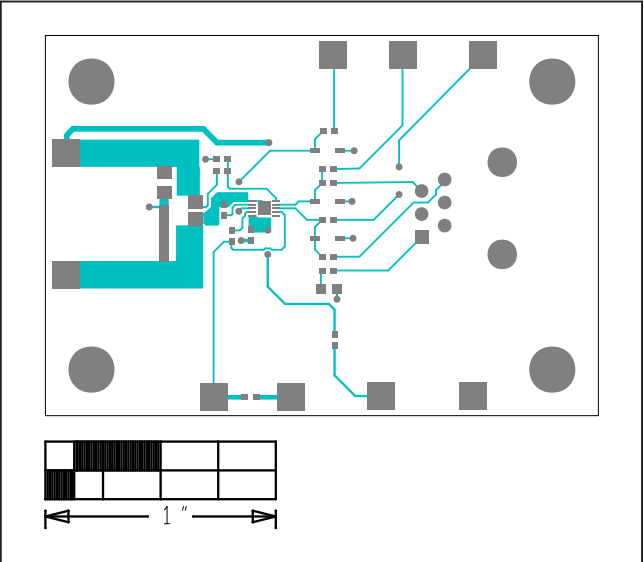
Top Layout
