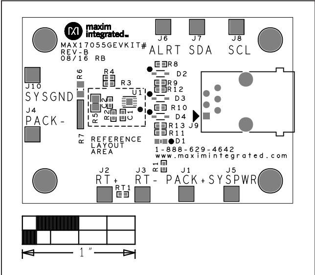
Component Placement
