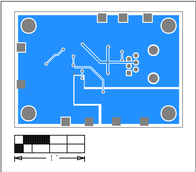
Bottom Layout
