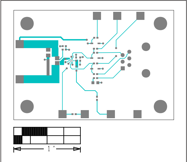
Top Layout
