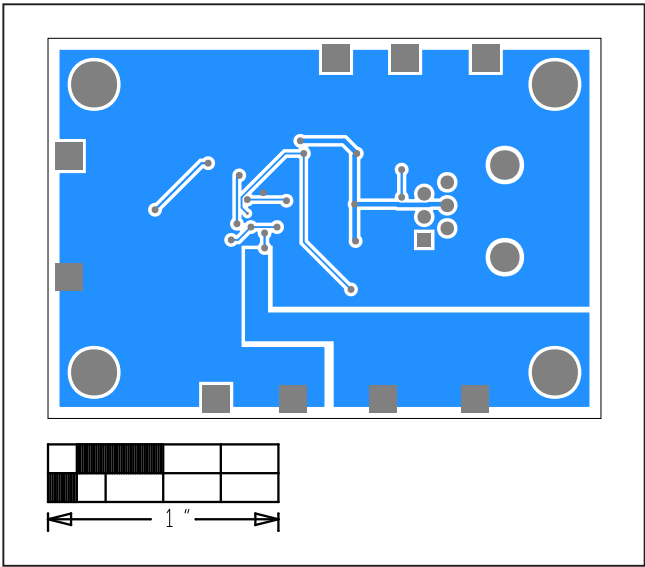
Bottom Layout
