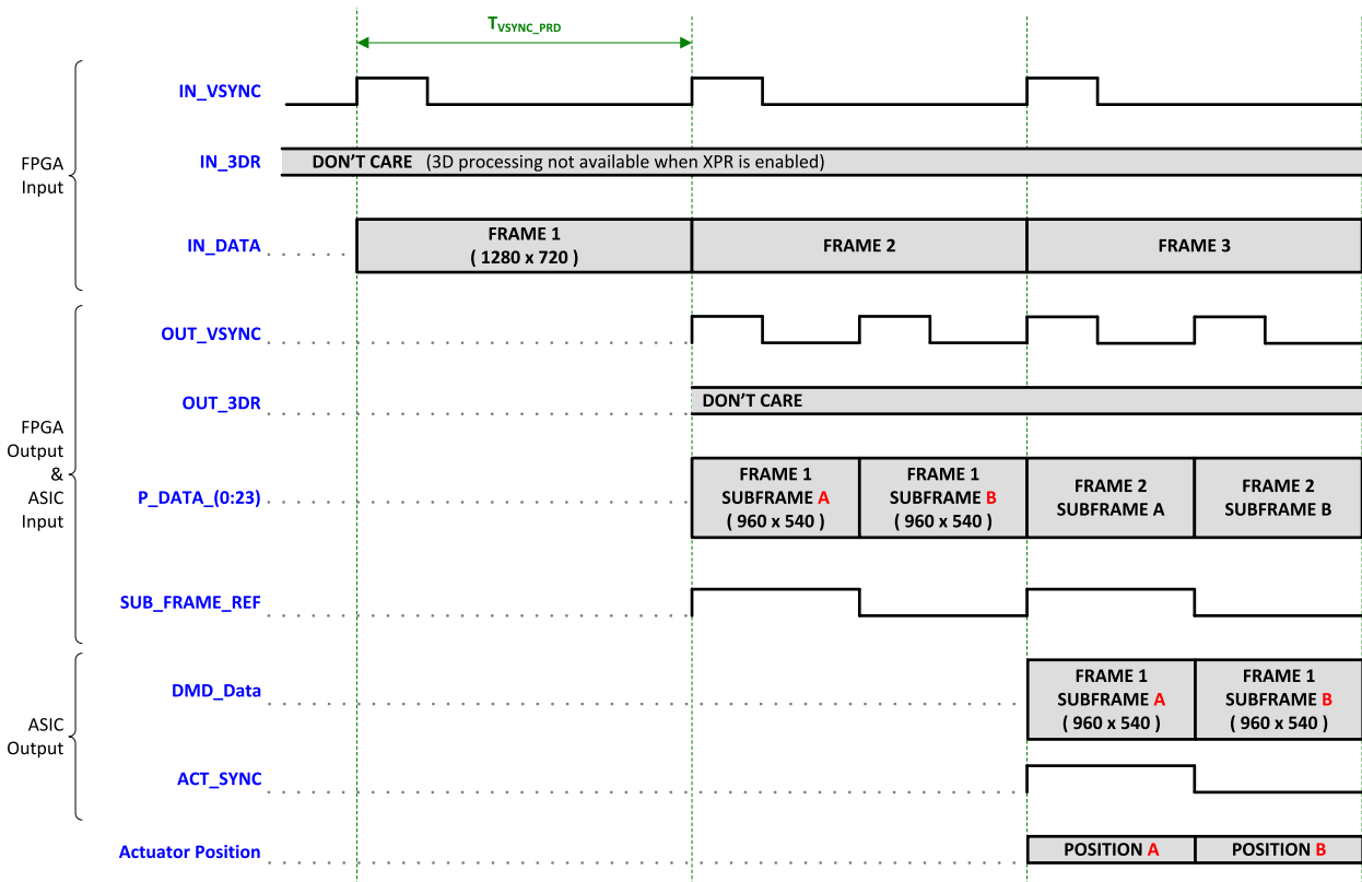
Figure 8. DLPC3434 2D Actuator Frame and Signal Timing
