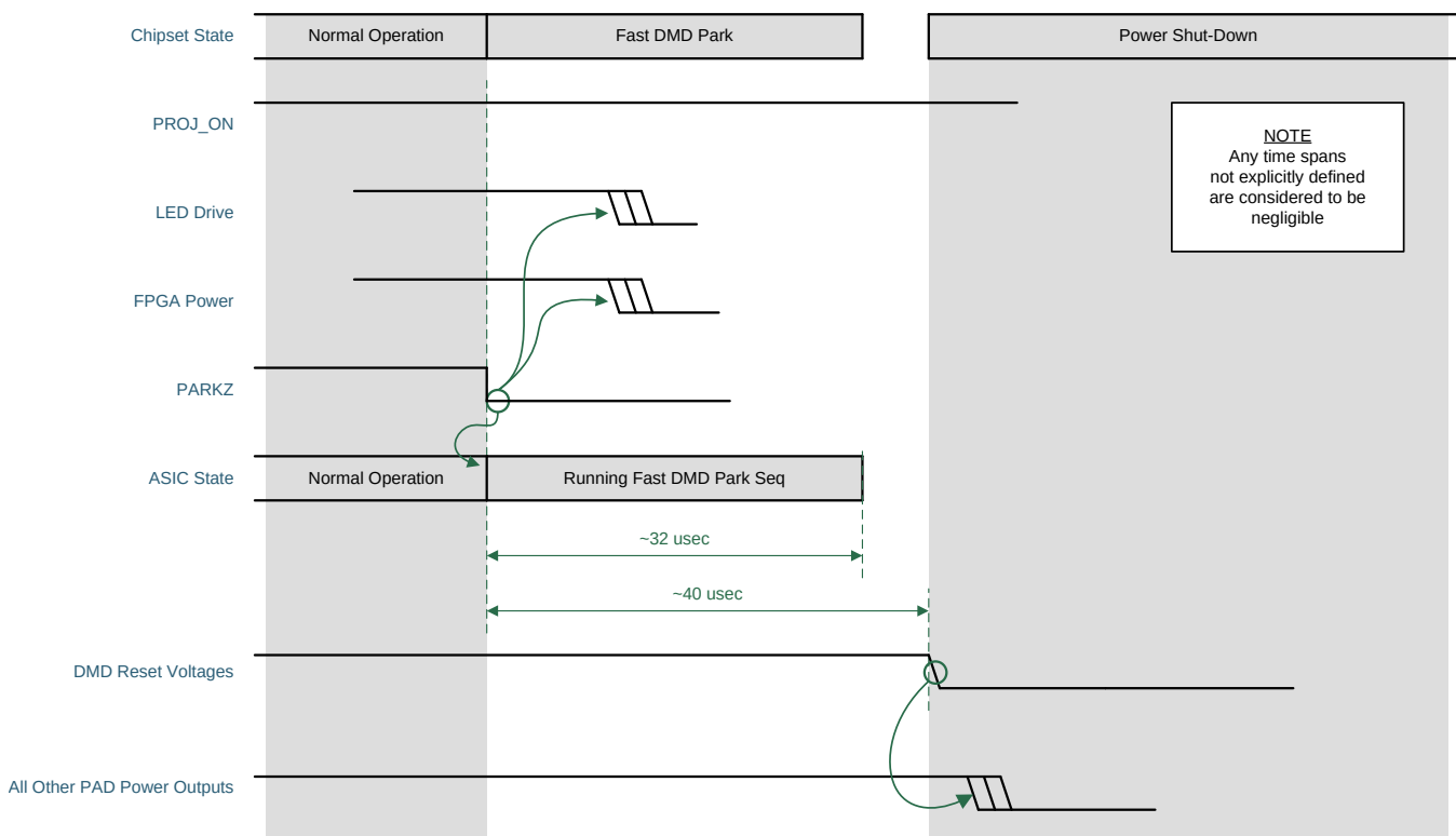
Figure 22. DLPC3434 Fast Power-Down
