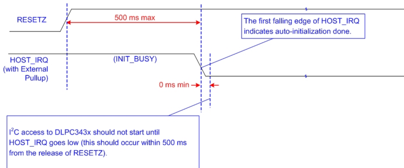
Figure 7. Host IRQ Timing
