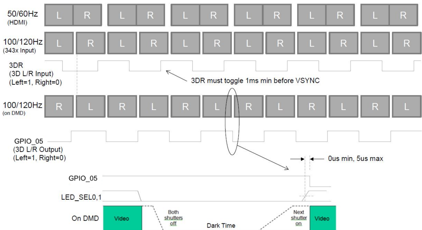
Figure 15. DLPC3434 L/R Frame and Signal Timing
