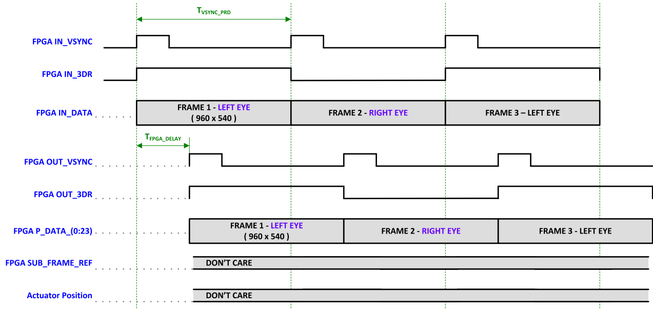
Figure 9. DLPC3434 3D Frame and Signal Timing
