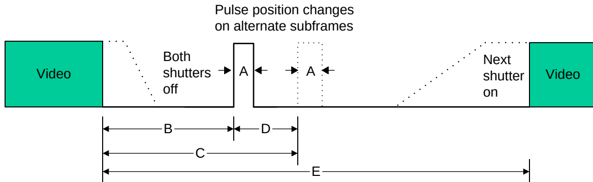
Figure 16. 3D DLP Link Pulse Timing
