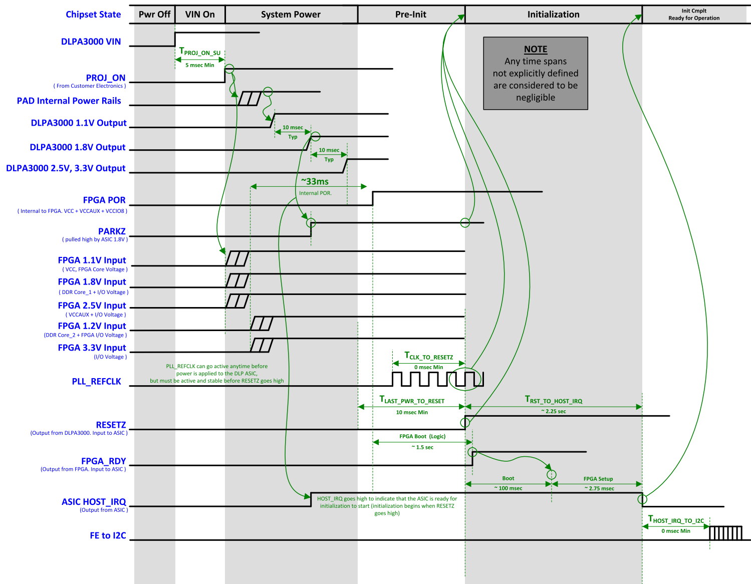
Figure 20. DLPC3434 Power-Up Timing
