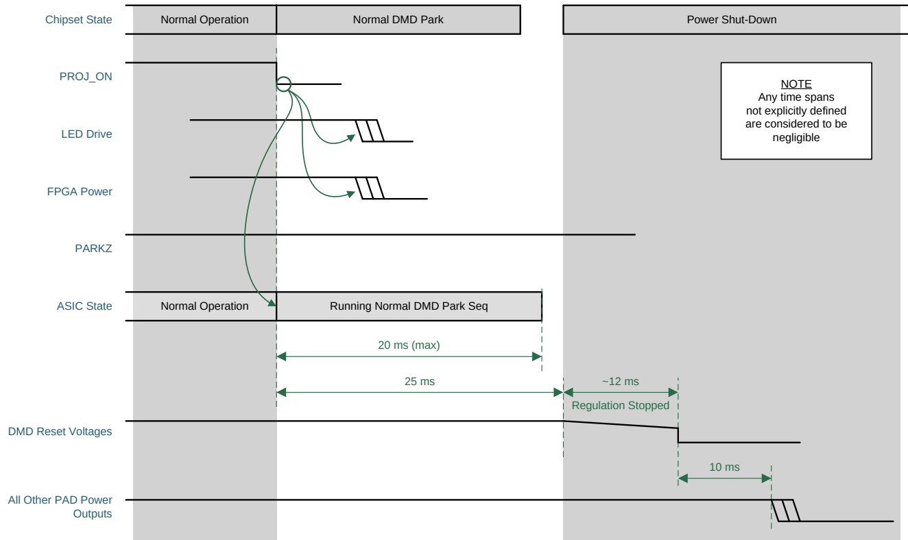
Figure 21. DLPC3434 Normal Power-Down
