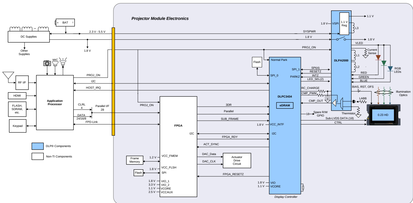
Figure 18. Typical Application Diagram
