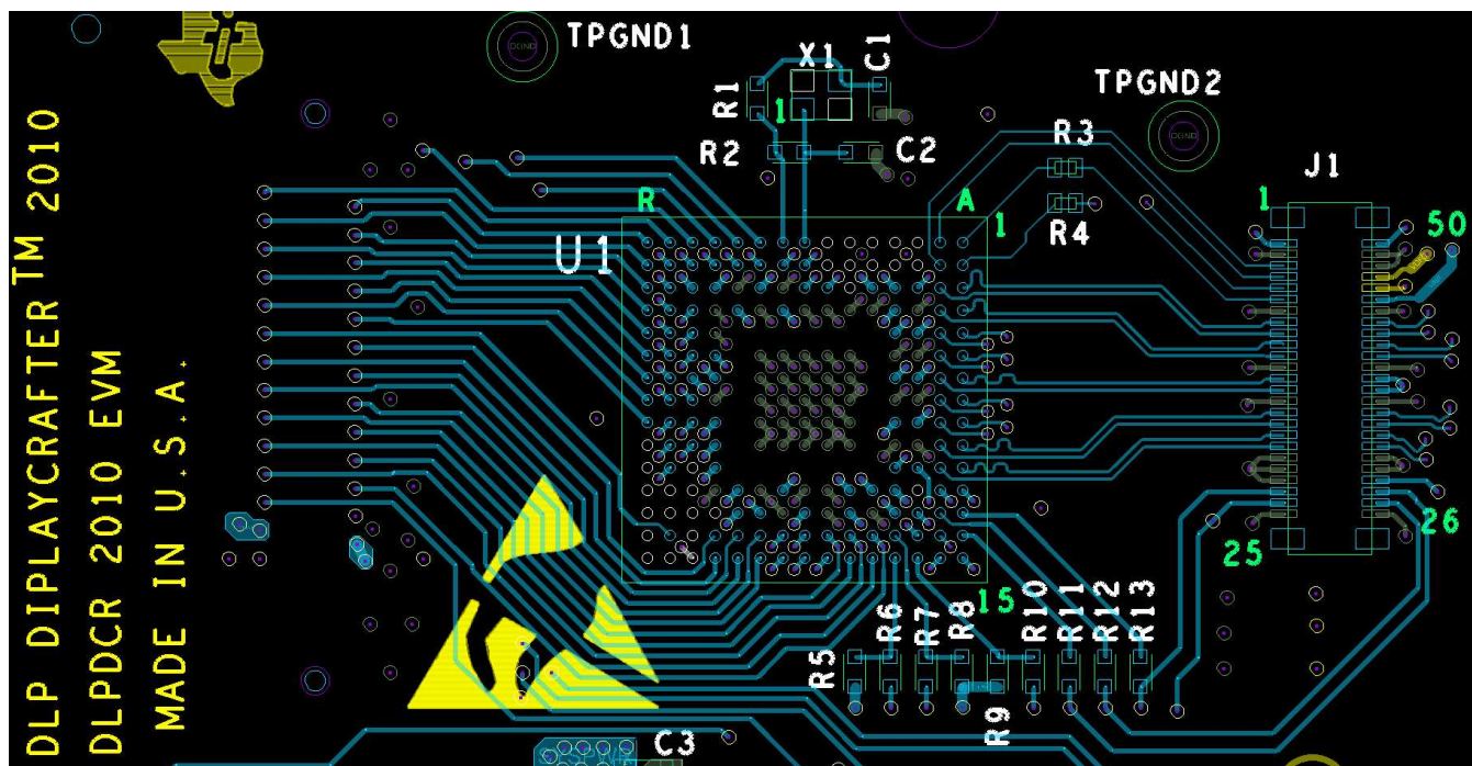
Figure 25. Layout Recommendation
