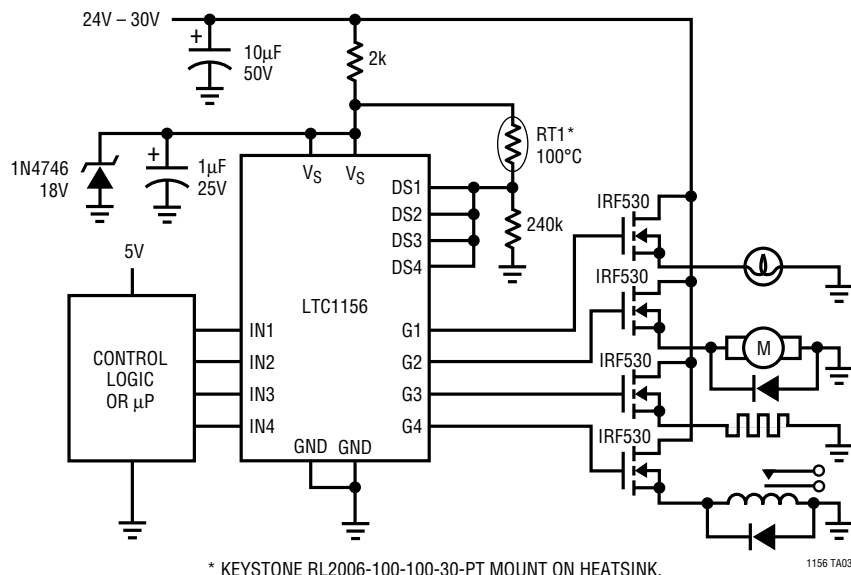
24V to 30V Quad Industrial Switch with Thermal Shutdown
