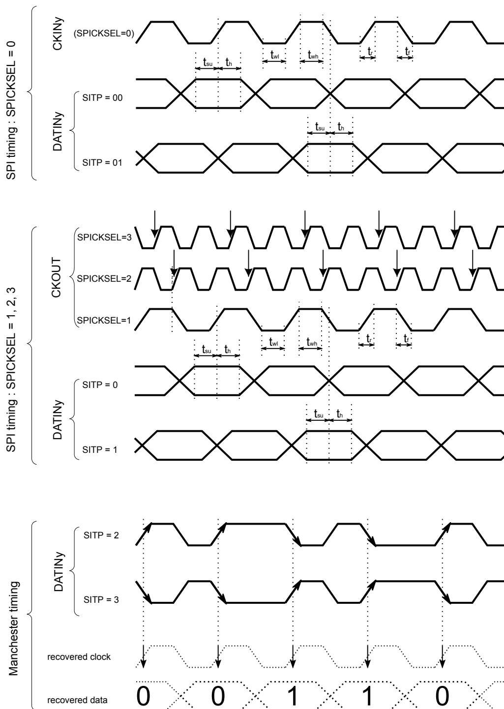
Figure 59. Channel transceiver timing diagrams
