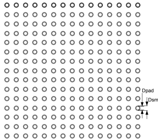
Figure 98. TFBGA - 225 balls, 13x13 mm, 0.8 mm pitch, thin profile fine pitch ball grid array package recommended footprint
