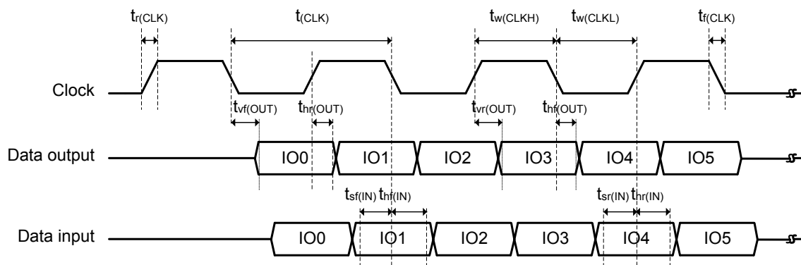
Figure 75. DDR mode
