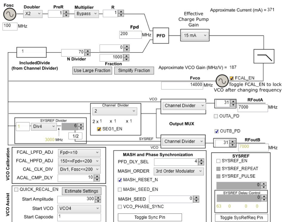
Figure 7. TICS Pro GUI LMX2594 Default Configuration
