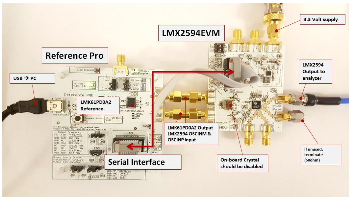
Figure 16. LMX2594EVM Setup With Reference Pro
