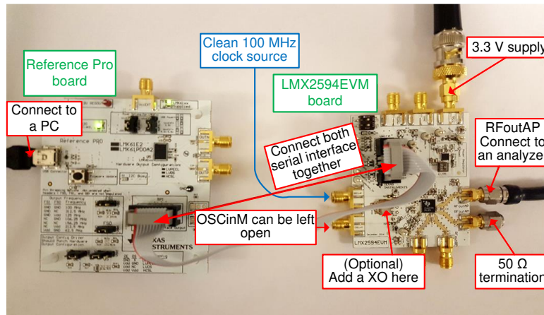
Figure 2. LMX2594EVM Setup
