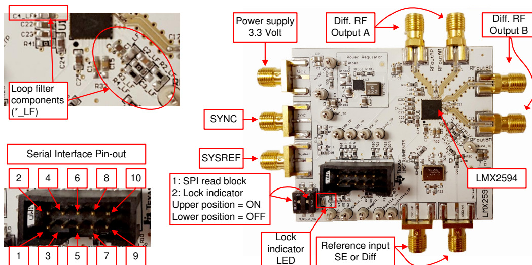
Figure 3. LMX2594EVM Description
