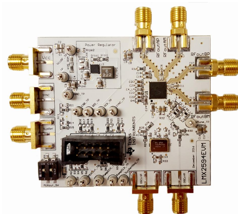
Figure 1. LMX2594EVM
