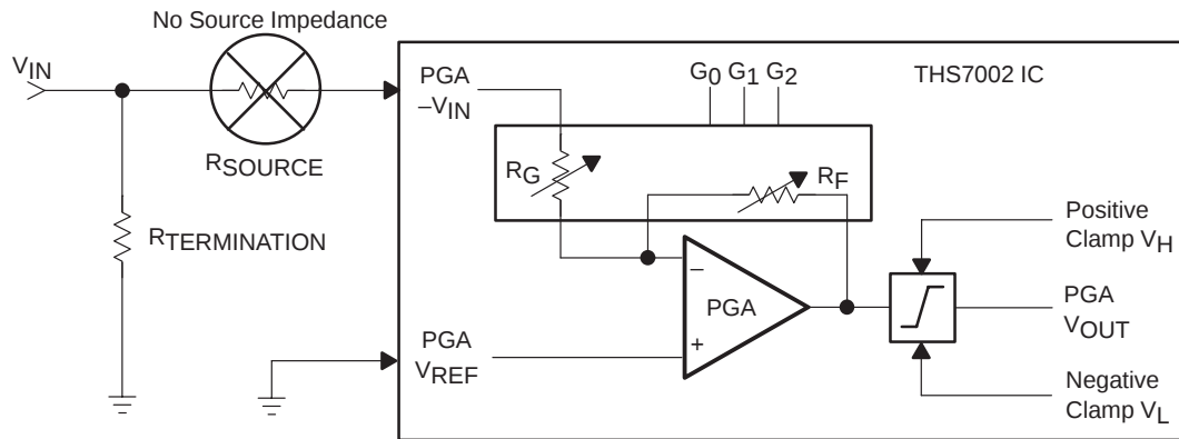
Figure 1–4. Simplified PGA Section of the THS7002
