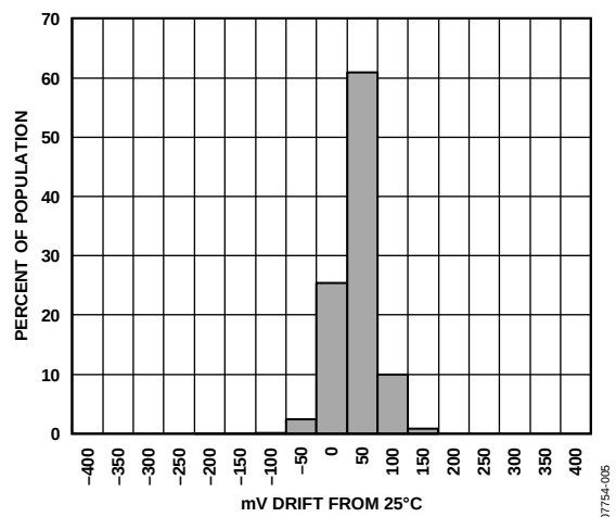
Figure 5. Null Drift over Temperature ( V_{RATIO} = 5 V )
