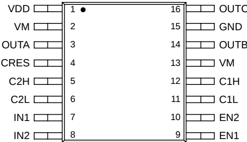
Figure 3. 17517 Pin Connections
