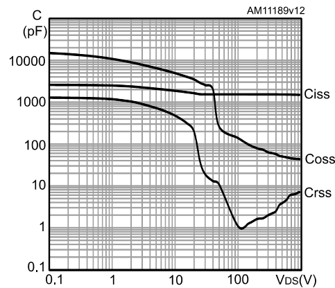
Figure 12: Capacitance variation
