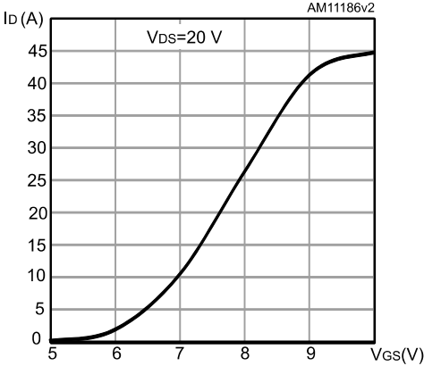
Figure 9: Transfer characteristics
