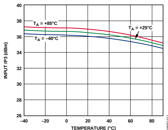
Figure 10. Input IP3 vs. Temperature
