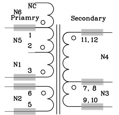
Note: ○ Winding start — Teflon tube a) Connection Diagram
