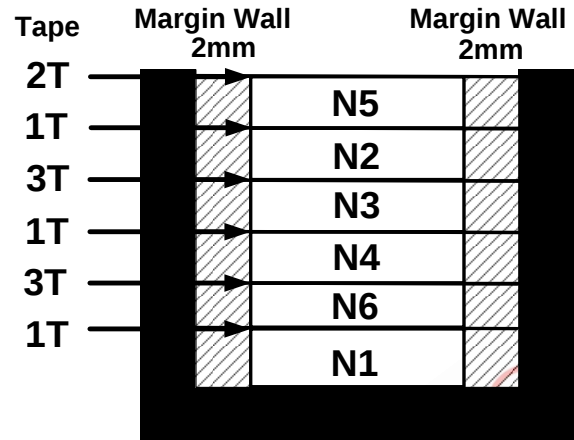
Bobbin b) Winding Diagram
