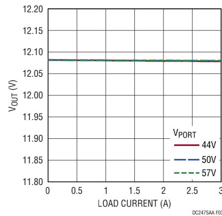
Figure 3. Load Regulation
