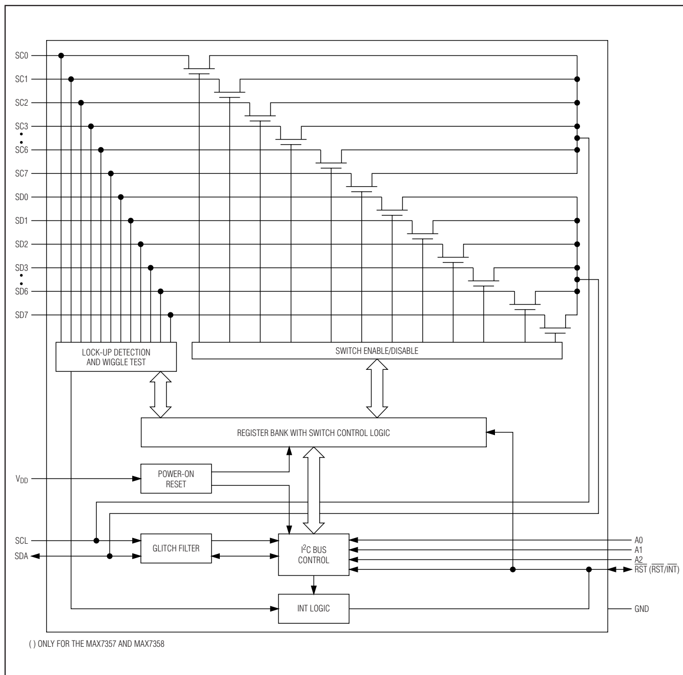
Functional Diagram
