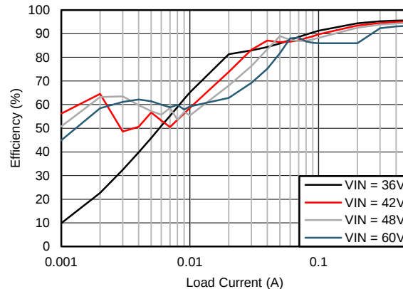
Figure 78. Efficiency
