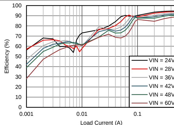
Figure 72. Efficiency
