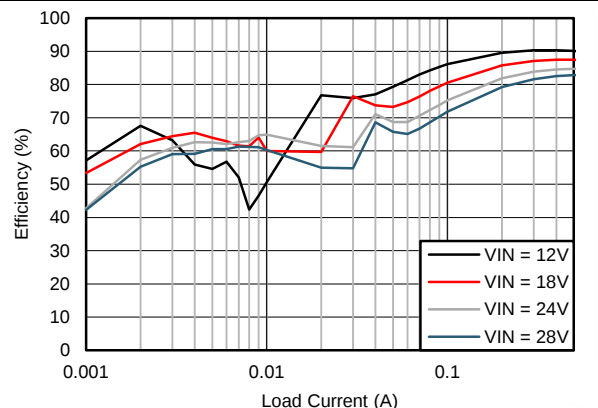
Figure 66. Efficiency
