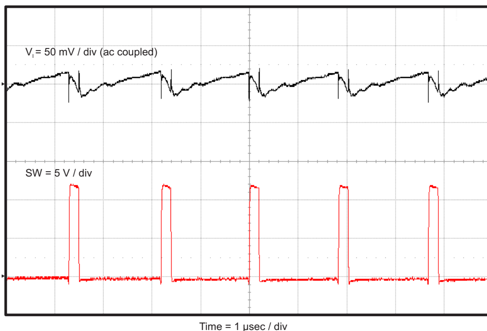
Figure 8. TPS562219AEMV-663 Input Voltage Ripple, I_{OUT} = 2 \text{ A}
