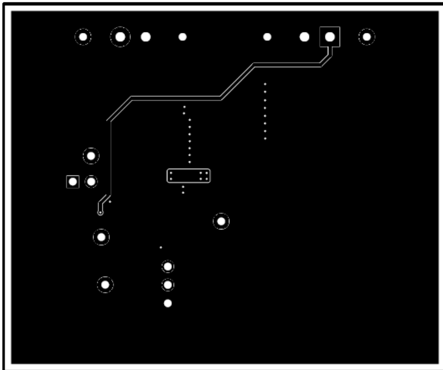
Figure 15. Bottom Layer
