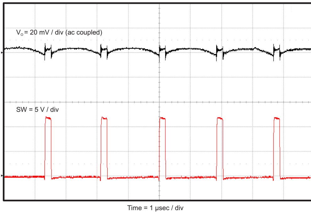
Figure 7. TPS562219AEMV-663 Output Voltage Ripple, I_{OUT} = 2 \text{ A}
