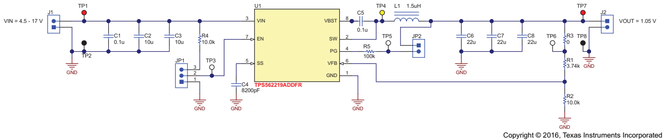
Figure 16. TPS562219AEM-663 Schematic Diagram
