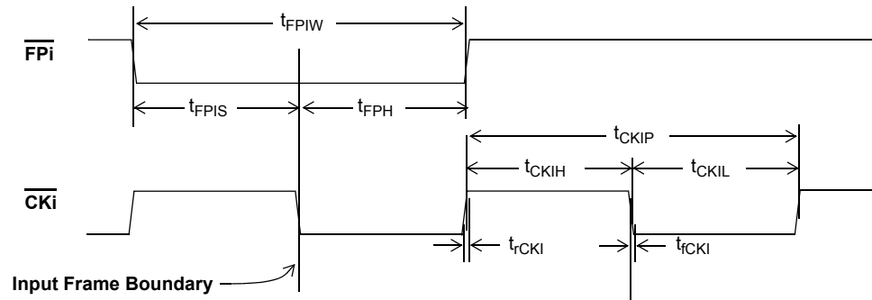
Figure 11 - Frame Pulse Input and Clock Input
