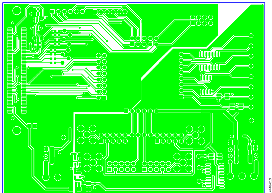
Figure 13. Motherboard Top Side Routing
