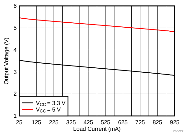
Figure 11. Output Voltage vs Load Current
