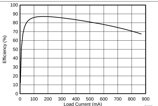
Figure 26. Efficiency vs Load Current
