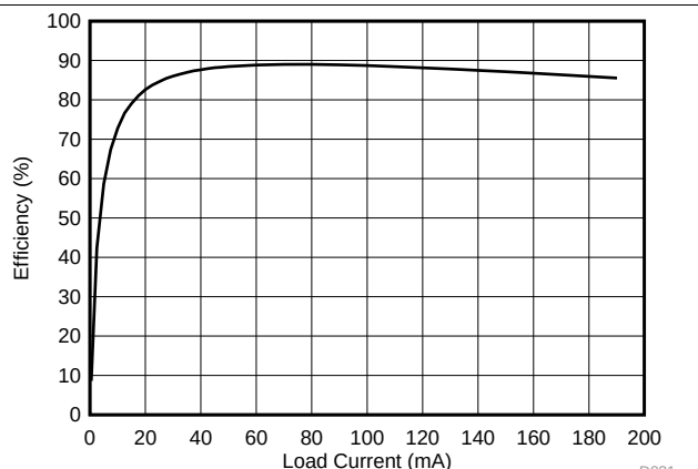
Figure 24. Efficiency vs Load Current
