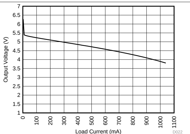
Figure 23. Output Voltage vs Load Current
