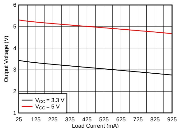
Figure 1. Output Voltage vs Load Current
