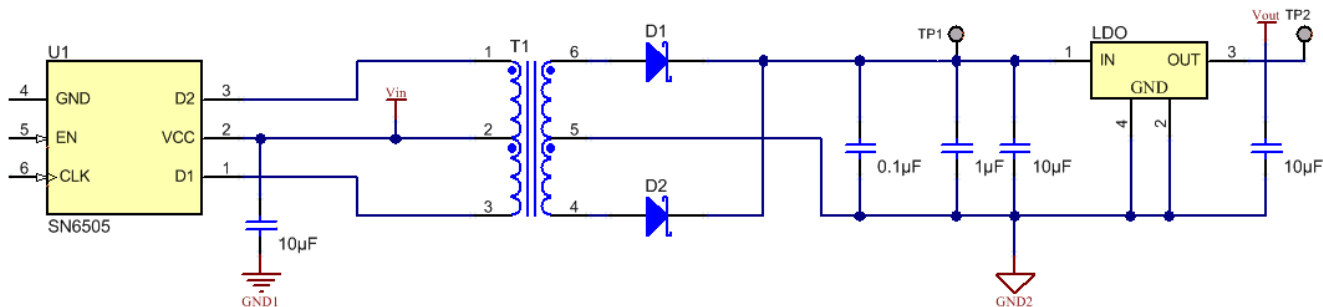
Figure 47. Regulated Output for Stable Supplies and High Current Loads
