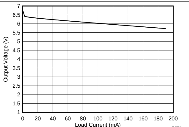
Figure 23. Output Voltage vs Load Current
