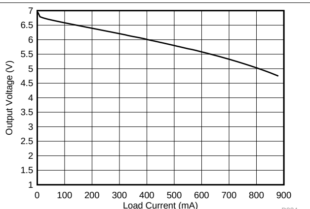
Figure 25. Output Voltage vs Load Current
