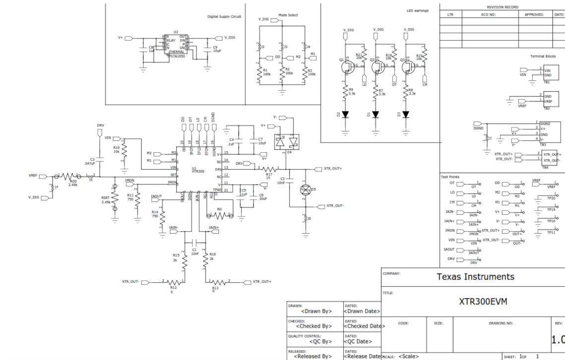
Figure 11. XTR300EVM Schematic
