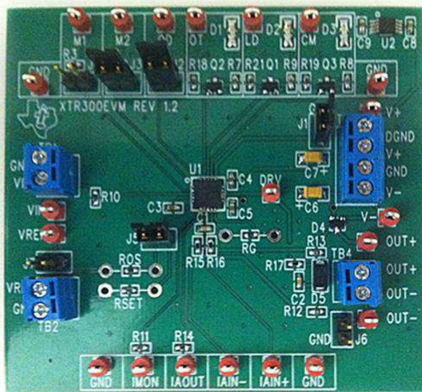
Figure 1. XTR300EVM
