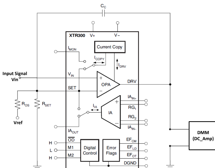
Figure 8. XTR300 Bidirectional Current Output Configuration Circuit Drawing
