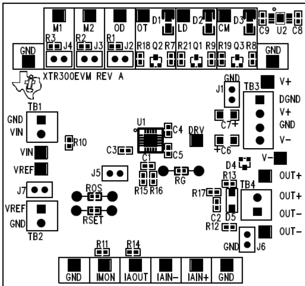
Figure 10. XTR300EVM Layout
