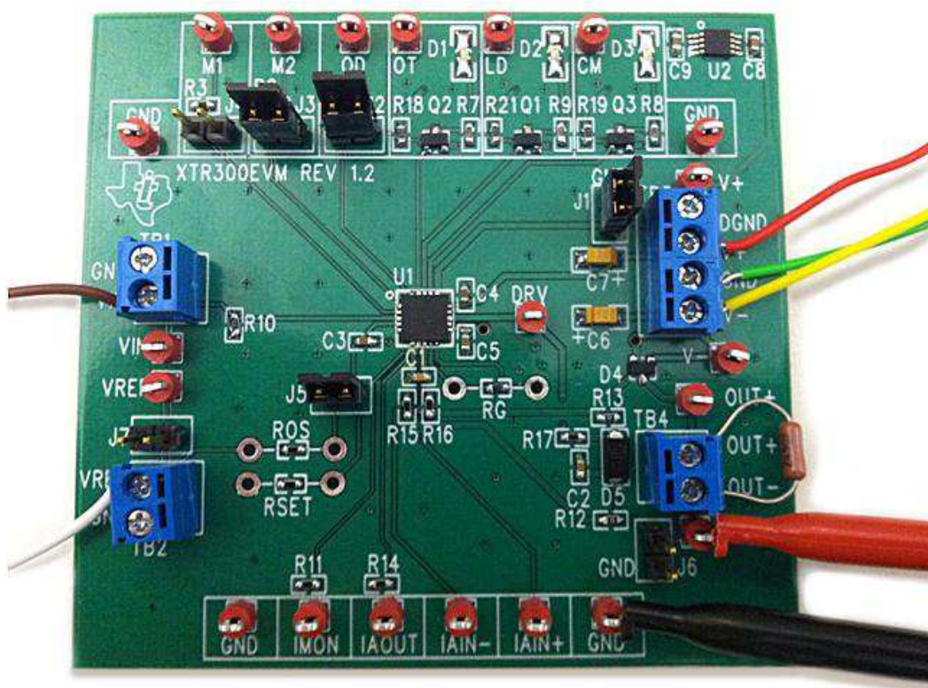
Figure 9. XTR300EVM Bidirectional Current Output Configuration Screenshot
