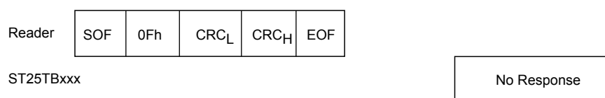
Figure 30. Completion frame exchange between reader and ST25TB512-AT
