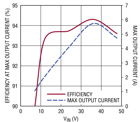
Max Output Current and Efficiency vs V IN
