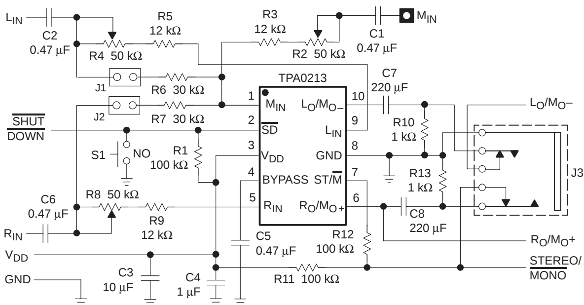
Figure 2–6. TPA0213 EVM Schematic Diagram
