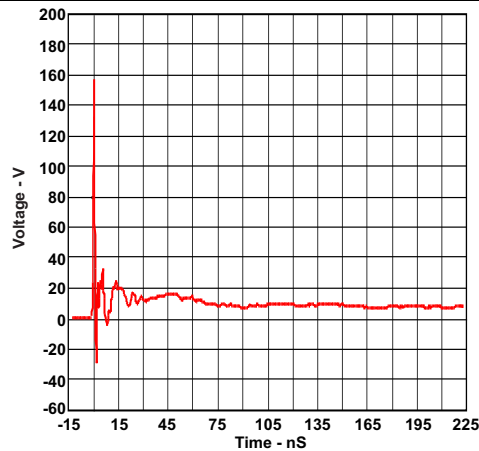
Figure 3. IEC Positive Clamping Waveform Using 8-kV Contact
