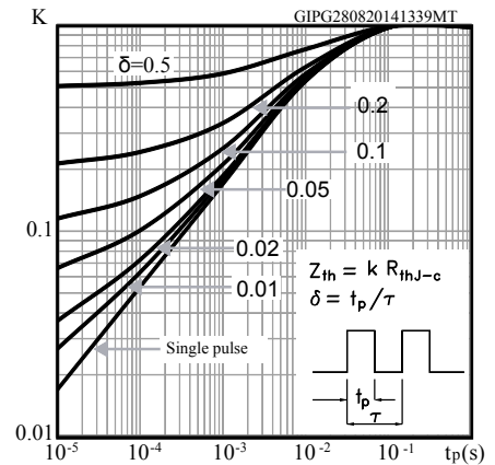
Figure 2. Thermal impedance
