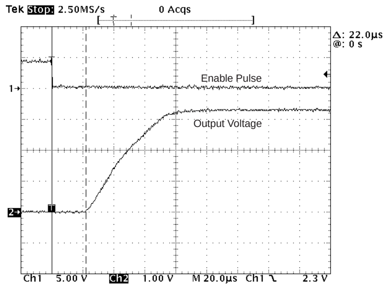
Figure 4–4. Delay Time EN → Output High
