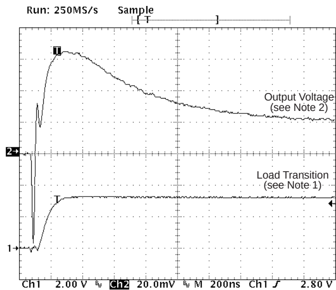
Figure 4–6. Full Load (100 mA) – No Load Transition With C_{out} = 10\text{ }\mu\text{F} Electrolytic
