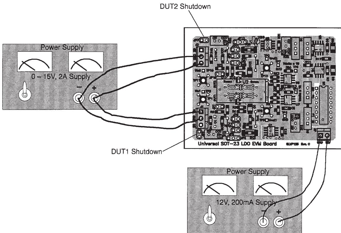
Figure 2–2. Test Setup
