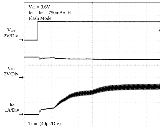
Figure 8 LX Current
