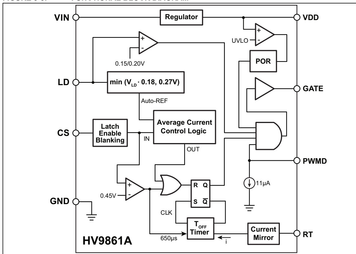
FIGURE 3-5: FUNCTIONAL BLOCK DIAGRAM
