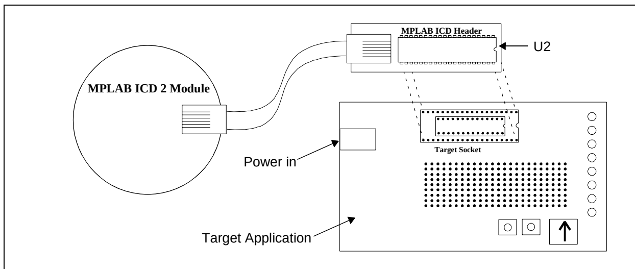
Figure 1: MPLAB ICD 2 Module Connection with Header
