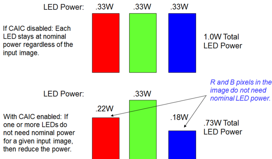
Figure 18. CAIC Power Reduction Mode (for Constant Brightness)
