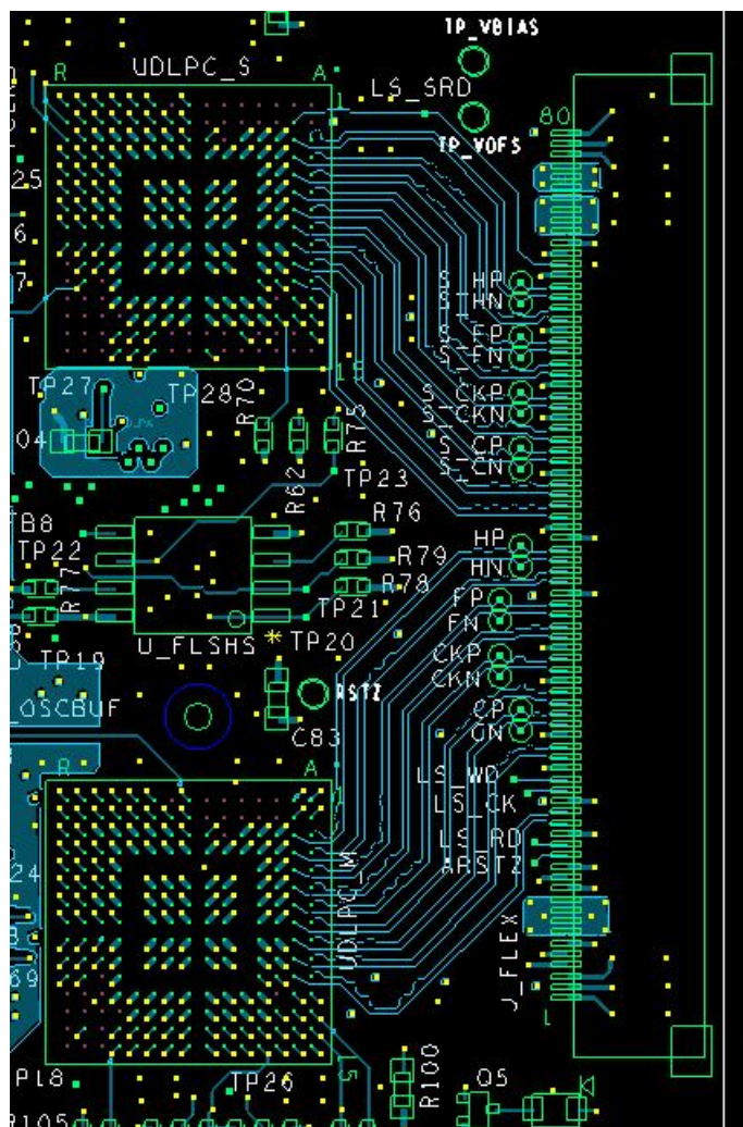
Figure 28. Board Layout
