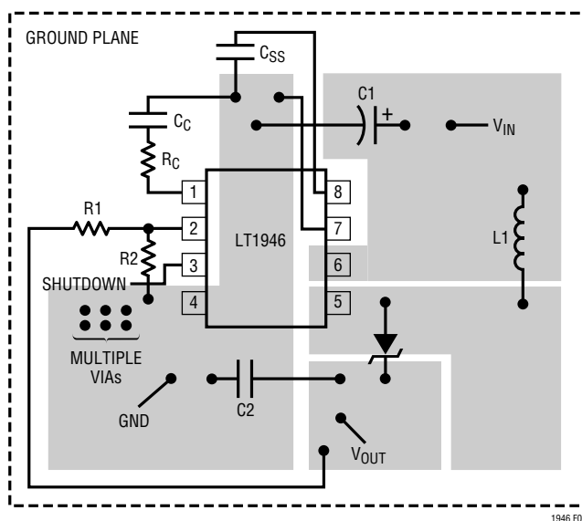
Figure 6. Recommended Component Placement for Boost Converter. Note Direct High Current Paths Using Wide PC Traces. Minimize Trace Area at Pin 1 ( V_C ) and Pin 2 (FB). Use Multiple Vias to Tie Pin 4 Copper to Ground Plane. Use Vias at One Location Only to Avoid Introducing Switching Currents Into the Ground Plane
