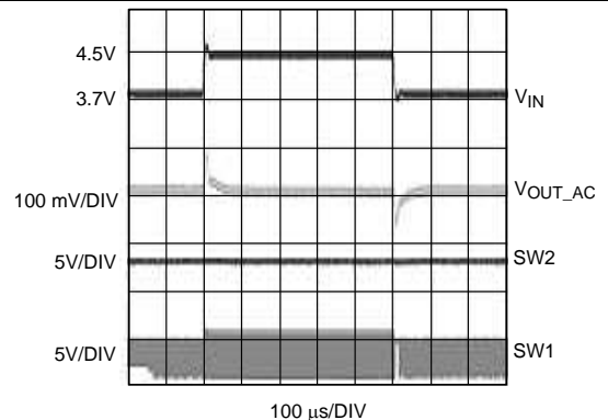
Figure 18. Line Transient in Buck Mode ( V_{OUT} = 3.4\text{ V} , Load = 500\text{ mA} )
