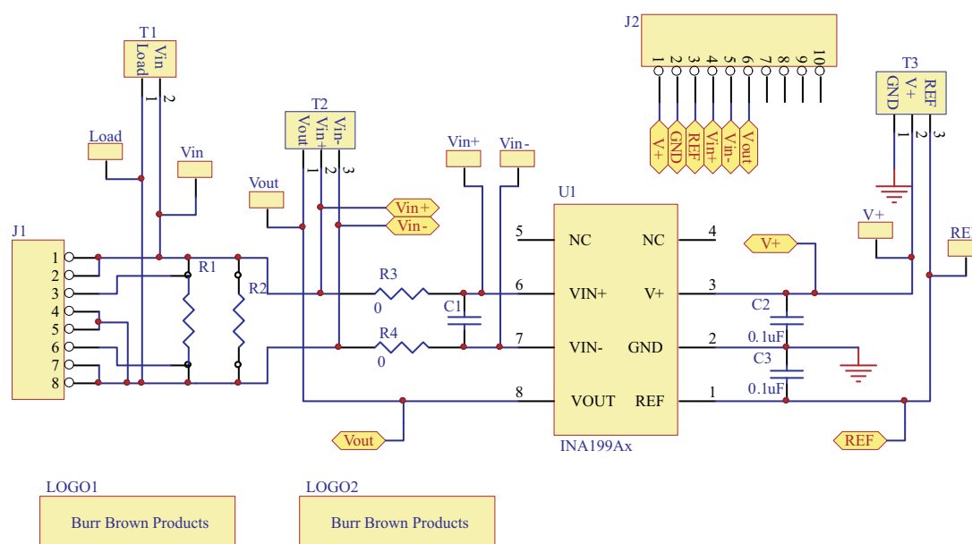
Figure 11. INA199A1-A3EVM Schematic
