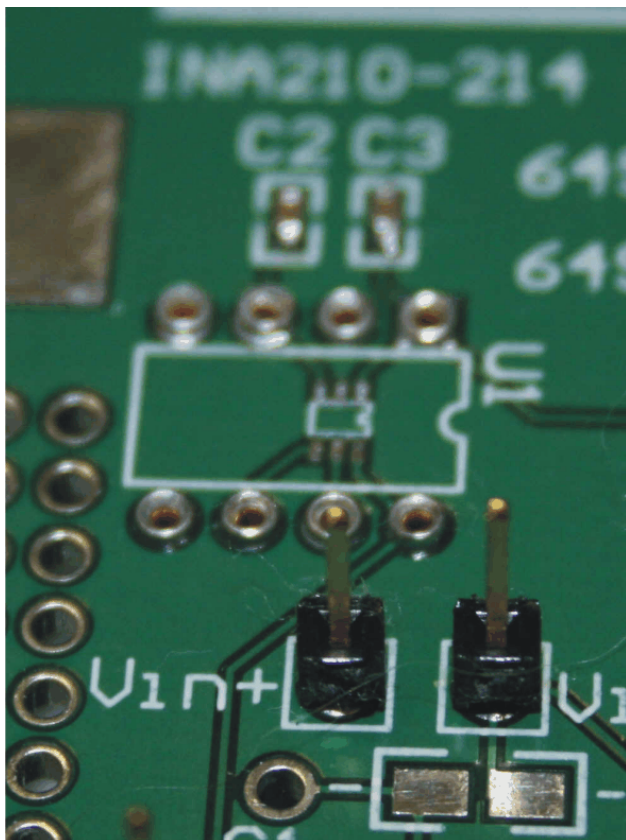
Figure 9. U1 Footprint
