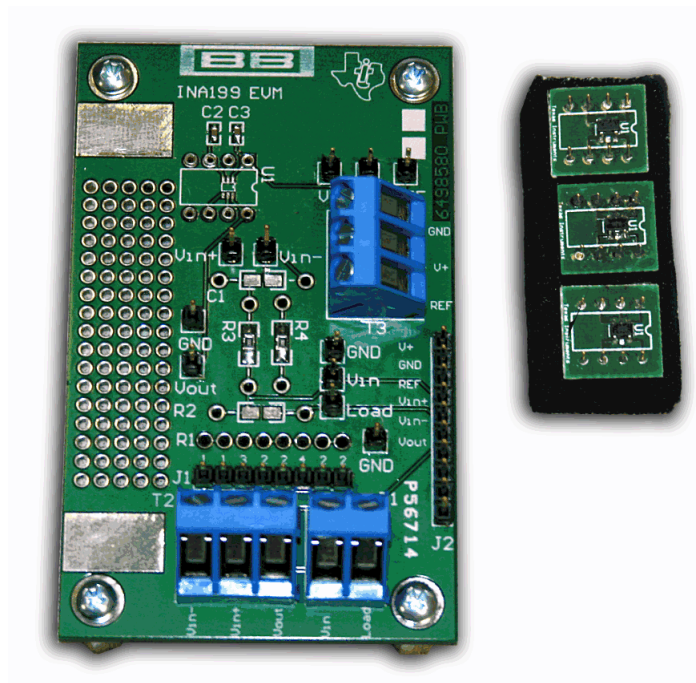
Figure 1. Hardware Included with the INA199A1-A3EVM
