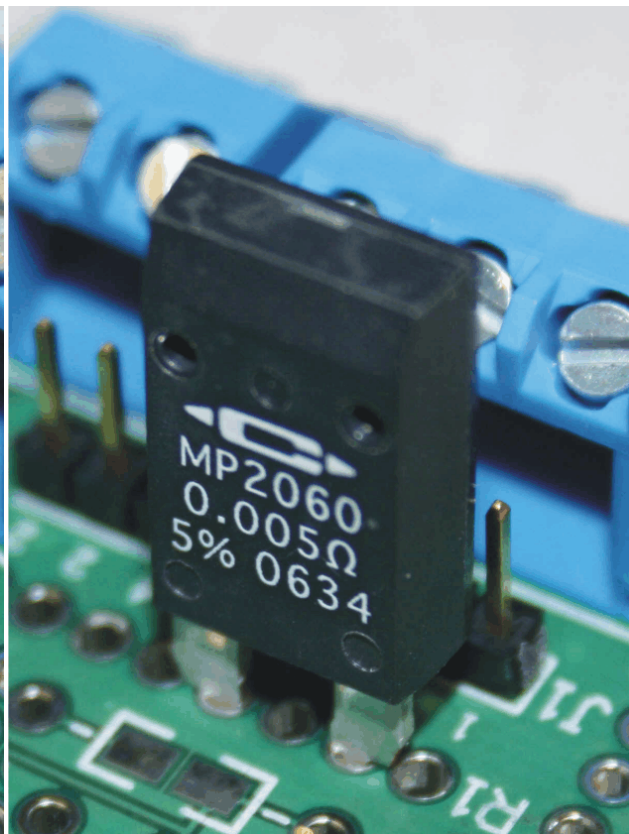
Figure 7. TO-220 Package in R1
