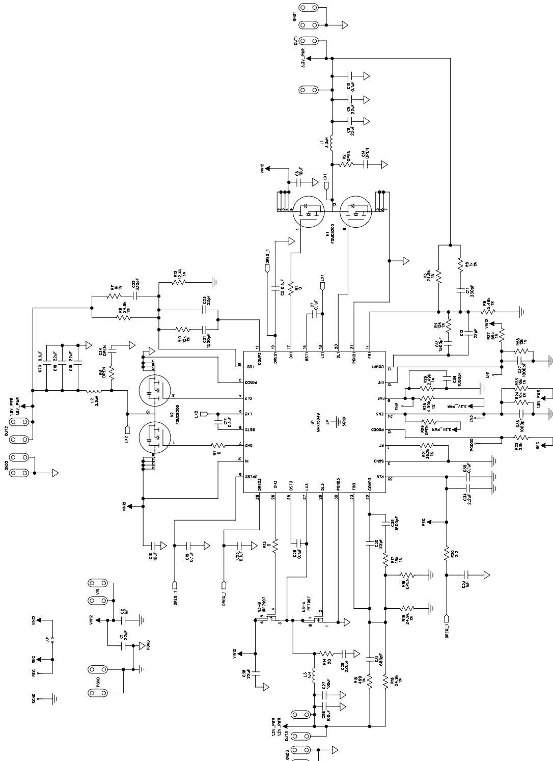
Figure 1. MAX15049 EV Kit Schematic
