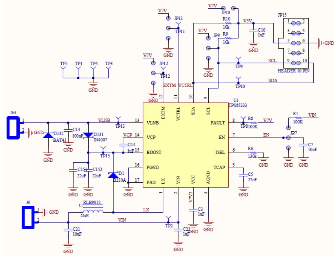
Figure 17. TPS65233EVM Schematic
