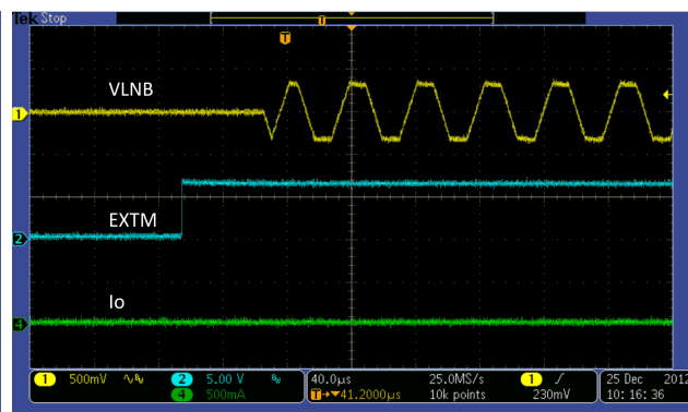
Figure 14. 22-kHz Tone Controlled by EXTM Logic Level, V_{IN} = 12\text{ V} , VLNB = 13.4\text{ V} , I_O = 0\text{ A}
