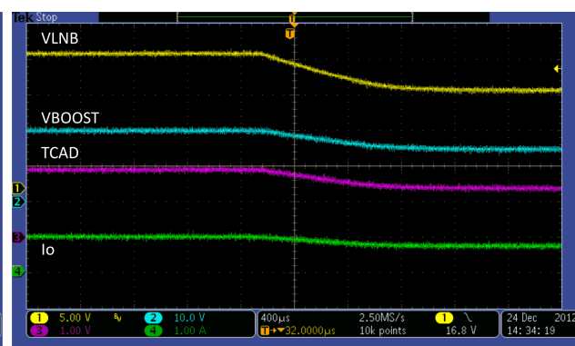
Figure 12. Voltage Transition, V_{IN} = 12\text{ V} , VLNB = 18.6\text{ V} to 13.4\text{ V} , I_O = 1\text{ A}
