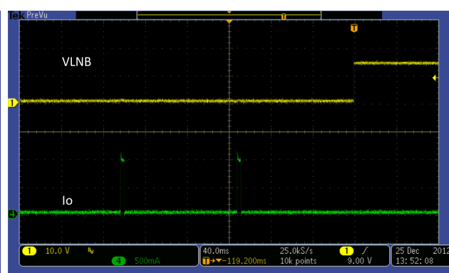
Figure 16. Output Hard Short and Recovery, V_{IN} = 12\text{ V} , VLNB = 13.4\text{ V}
