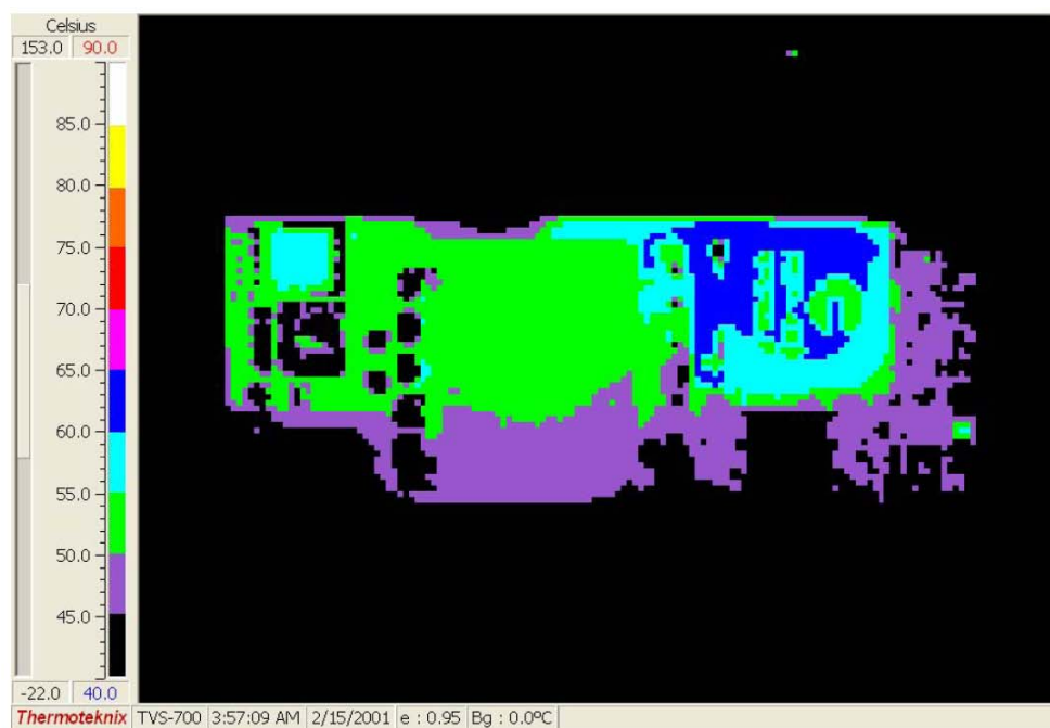
Figure 6. Thermal Map, Frontside at 18Vin and 10Aout (Ta = 25 degrees C)
