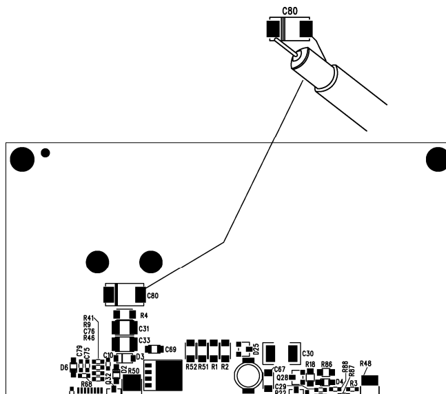
Figure 1. Proper Measurement Equipment Setup
