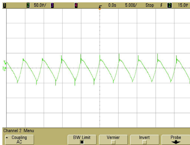
Figure 4. Output Ripple at 18Vin and 10Aout (25MHz) (50mV, 5us / div, 25MHz)
