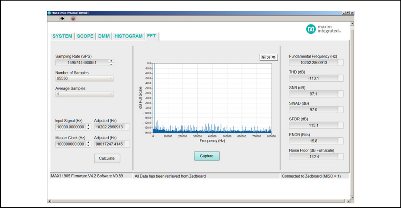
Figure 10. MAX11905 FFT ( f_{\text{SAMPLE}} = 1.6\text{Msps} , f_{\text{IN}} = 10\text{kHz} )
