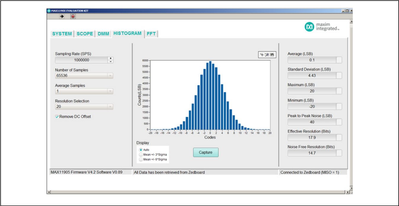
Figure 11. MAX11905 Output Data Histogram (Inputs Shorted, Averaging = 1, f_{\text{SAMPLE}} = 1\text{Msps} )
