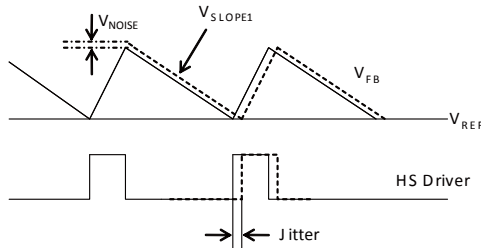
Figure 4: Jitter in PWM Mode
