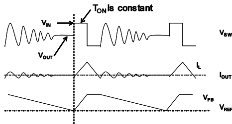
Figure 3: Light-Load Operation
