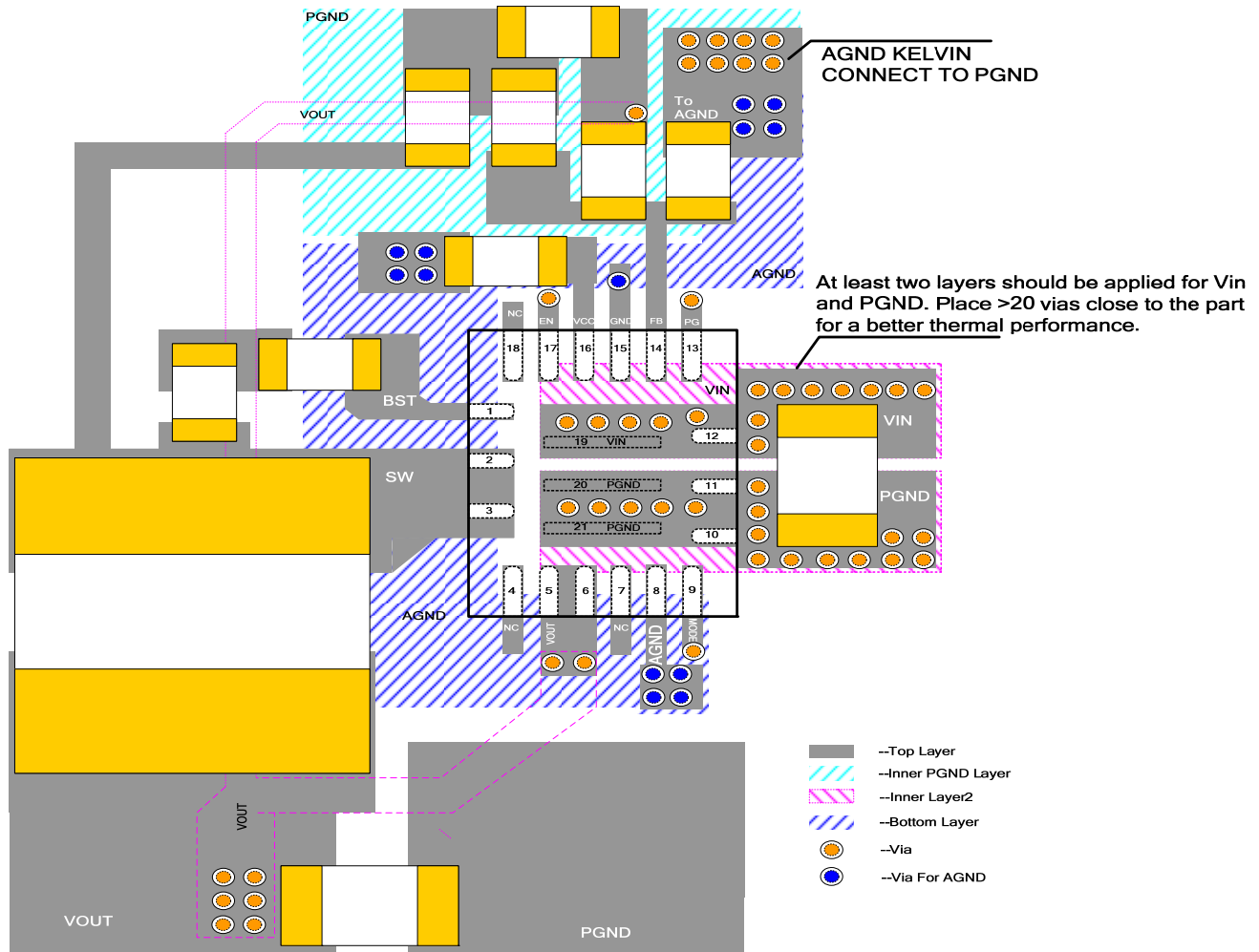
Figure 13: Recommended Layout
