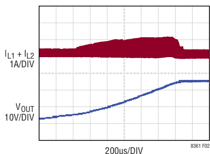
Figure 3. Soft-Start Waveforms
