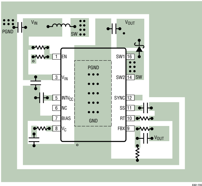
Figure 5. Suggested Boost Converter Layout
