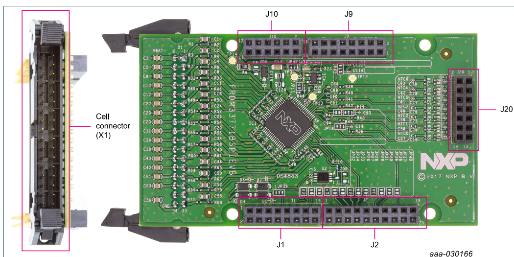
Figure 5. Connectors
