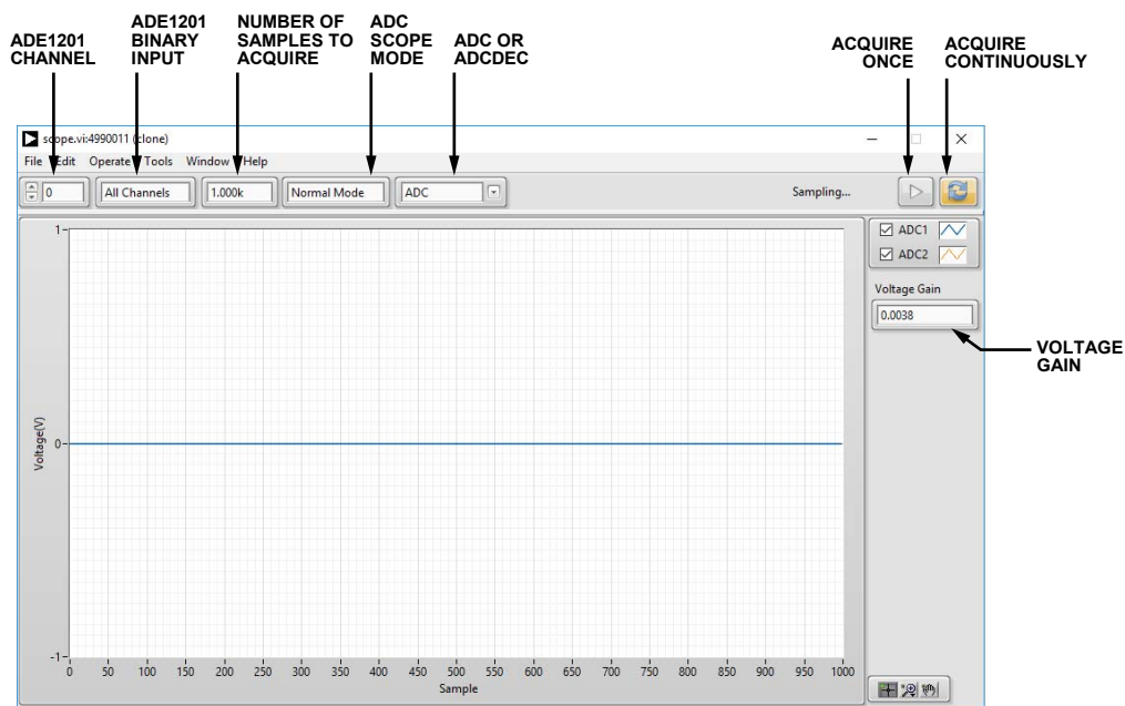
Figure 9. ADC Scope Window
