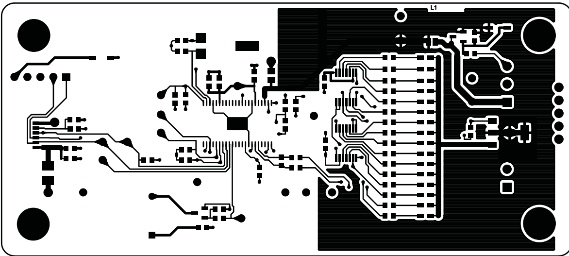
Figure 15. HPA615A Layer 1
