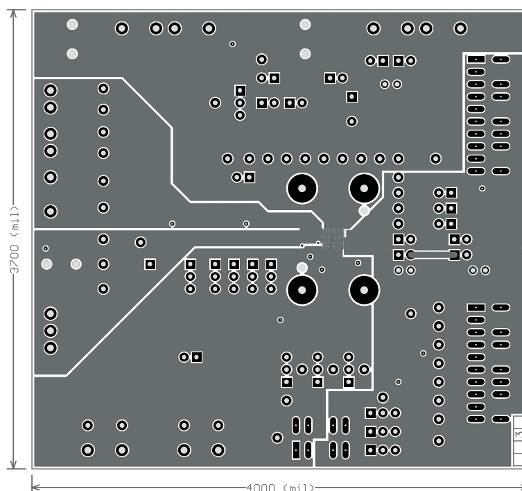
Figure 24. Mid-Layer 2
