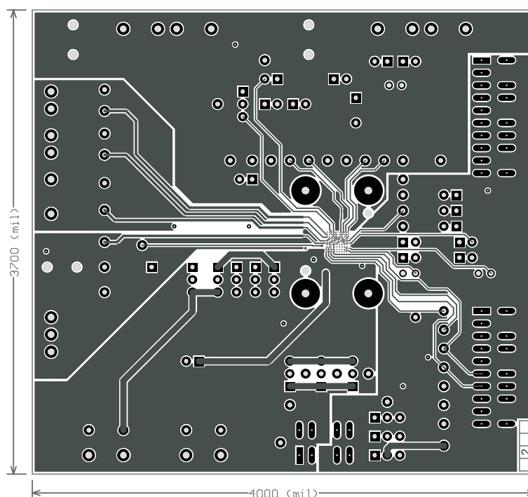
Figure 23. Mid-Layer 1
