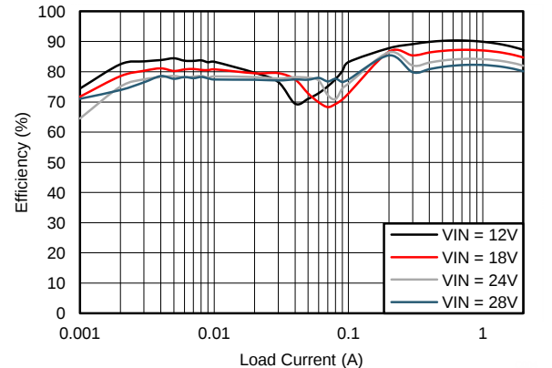
Figure 66. Efficiency
