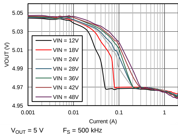
Figure 9. V_{OUT} Regulation
