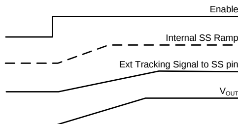
Figure 38. Tracking With Longer Start-up Time Than Tthe Internal Ramp
