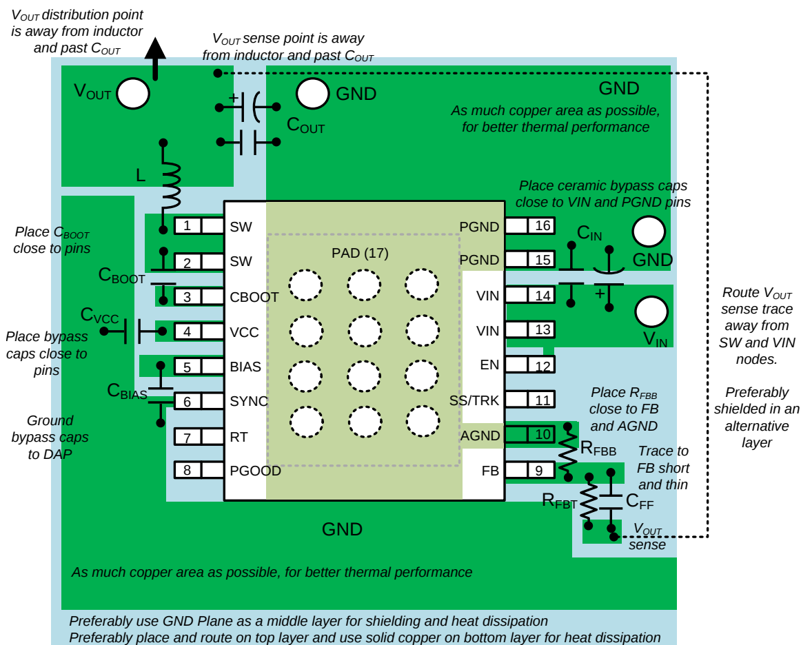
Figure 102. LM46002-Q1 PCB Layout Example and Guidelines
