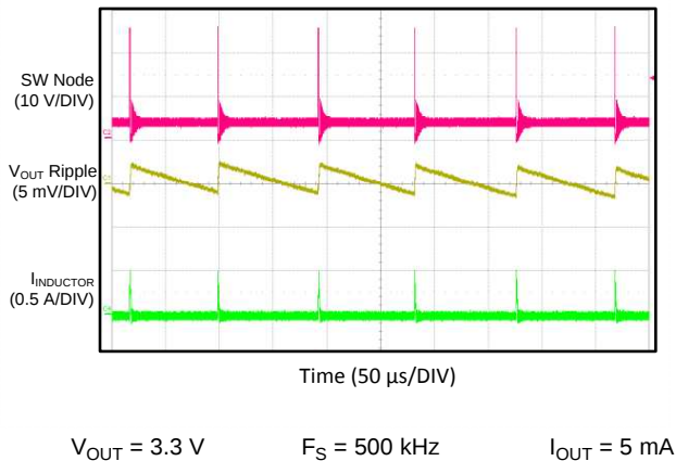
Figure 91. Switching Waveform in PFM Operation
