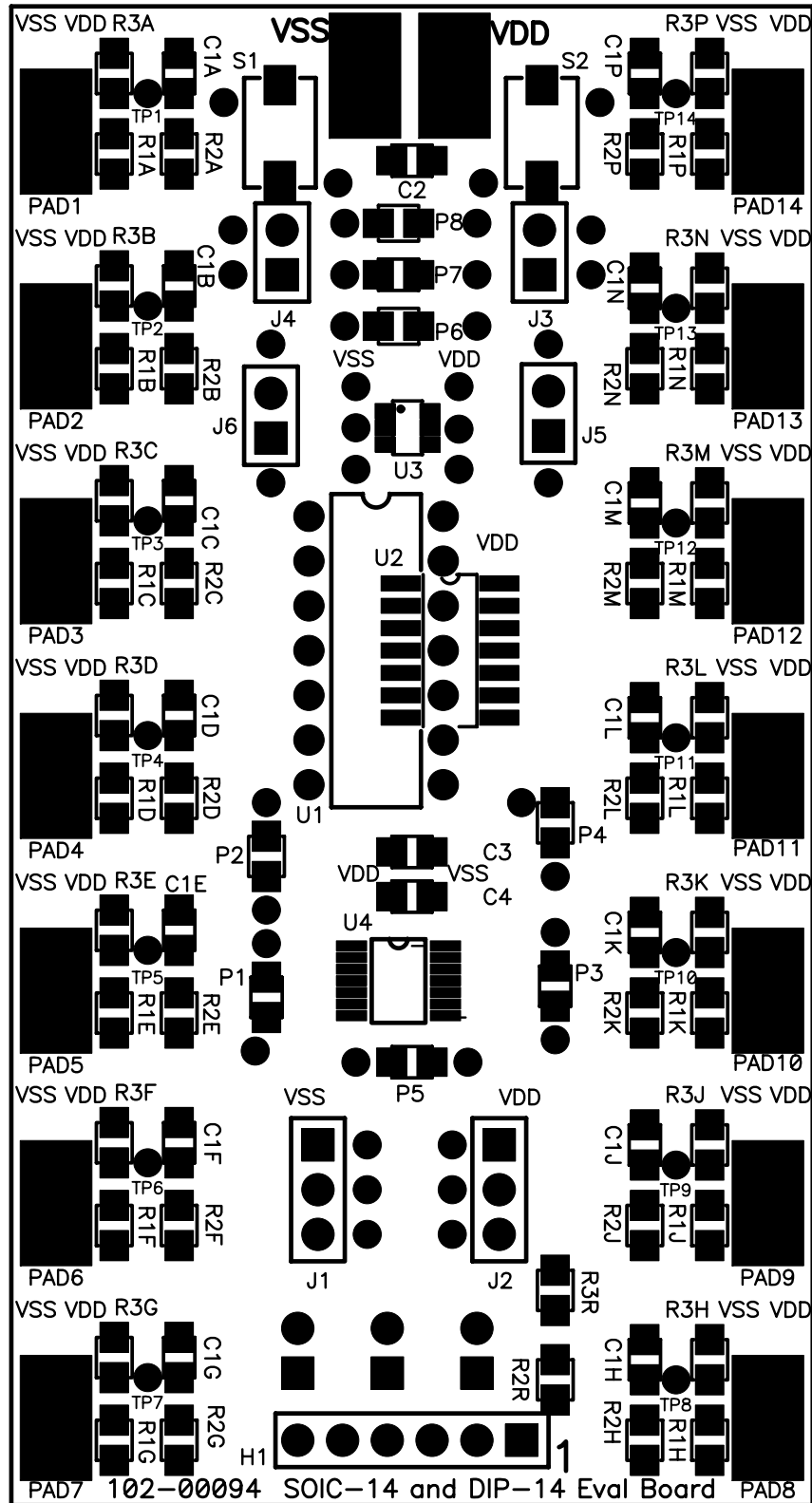
FIGURE A-9: Board Layout – Component Layer.
