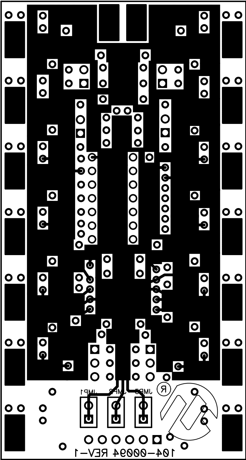
FIGURE A-10: Board Layout – Bottom Silk.
