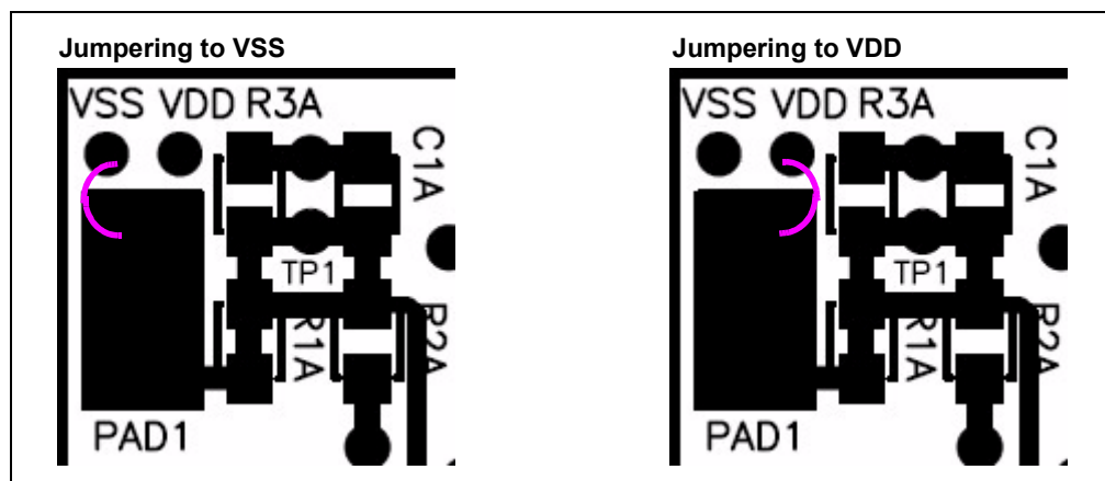
FIGURE 2-4: Jumpering the PCB pad to either VDD or VSS.
