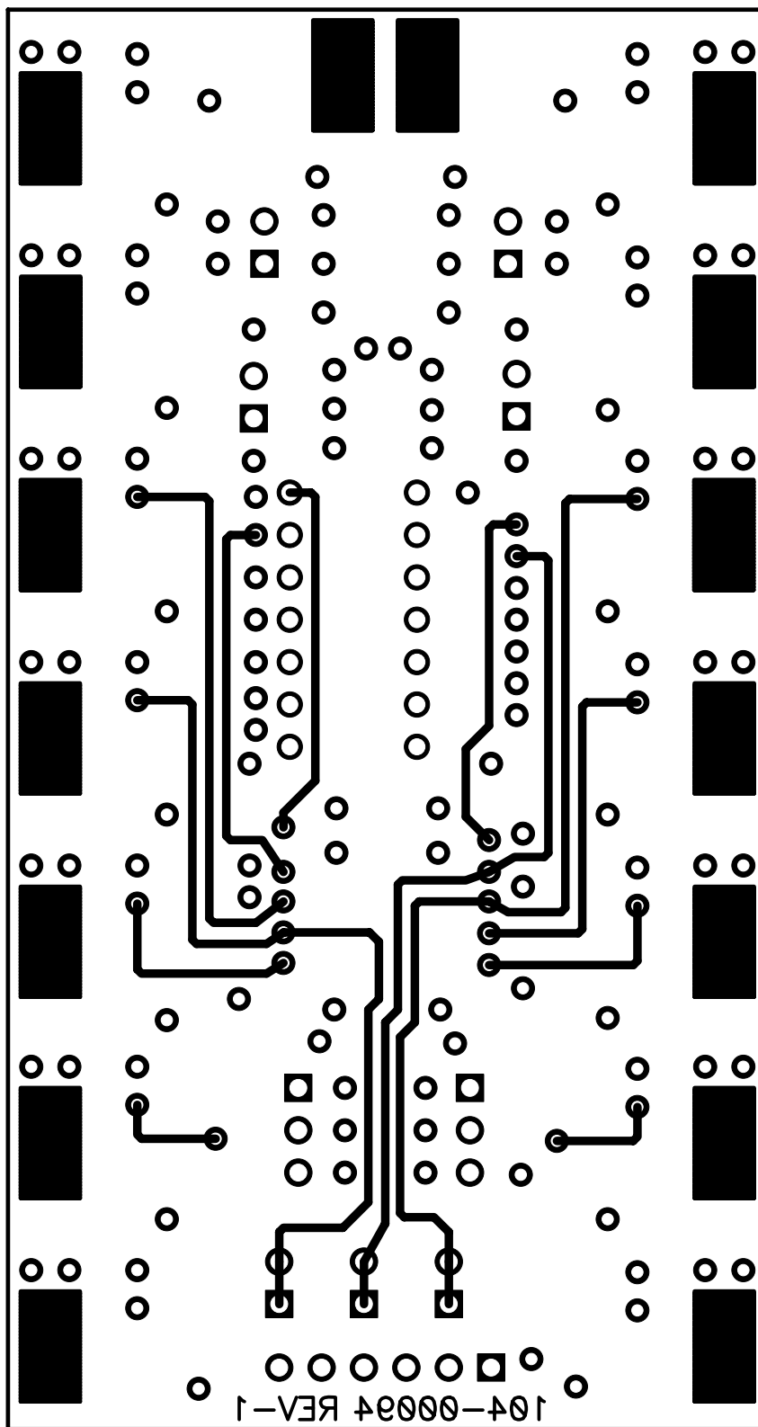
FIGURE A-6: Board Layout – Bottom Layer.
