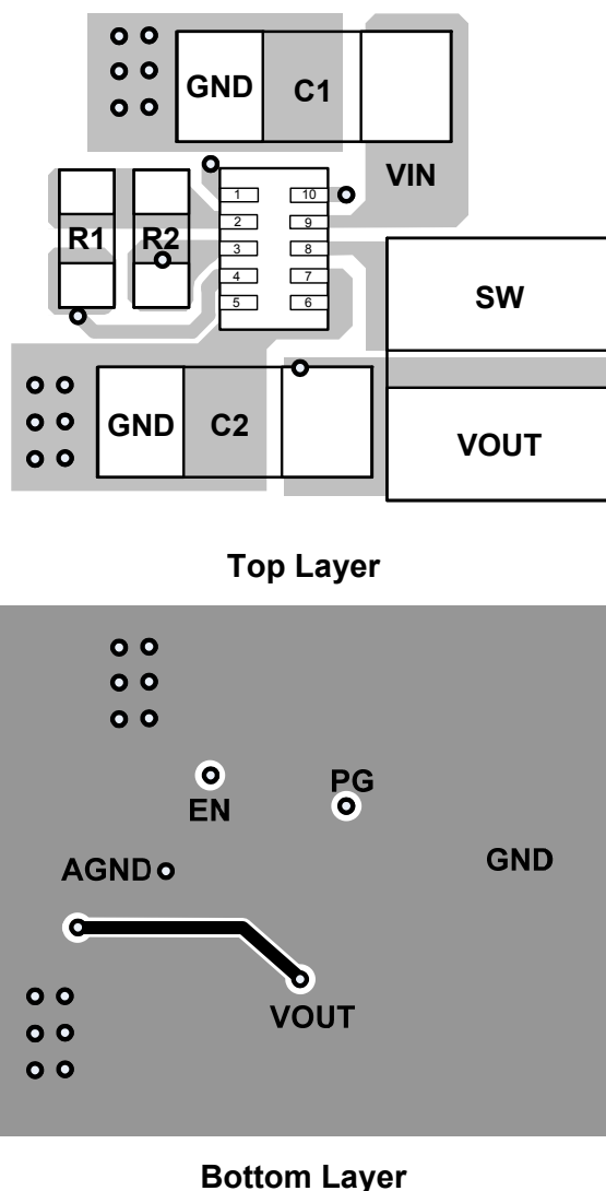
Figure 3: Layout Recommendation
