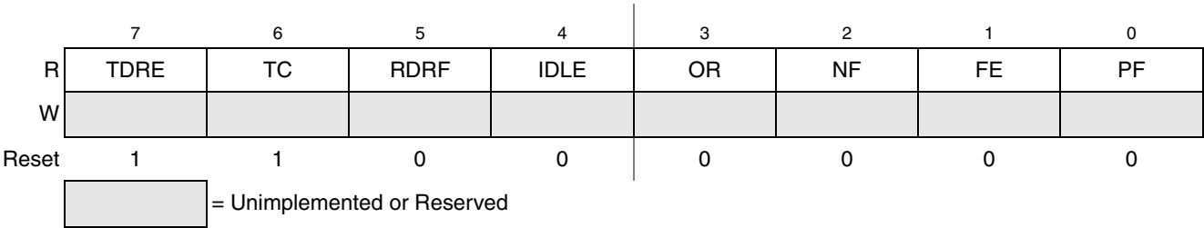
Figure 10-8. SCI Status Register 1 (SCIS1)
