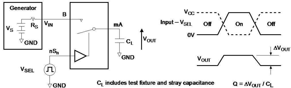
Figure 14. Charge Injection Test
