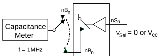
Figure 15. Channel Off Capacitance
