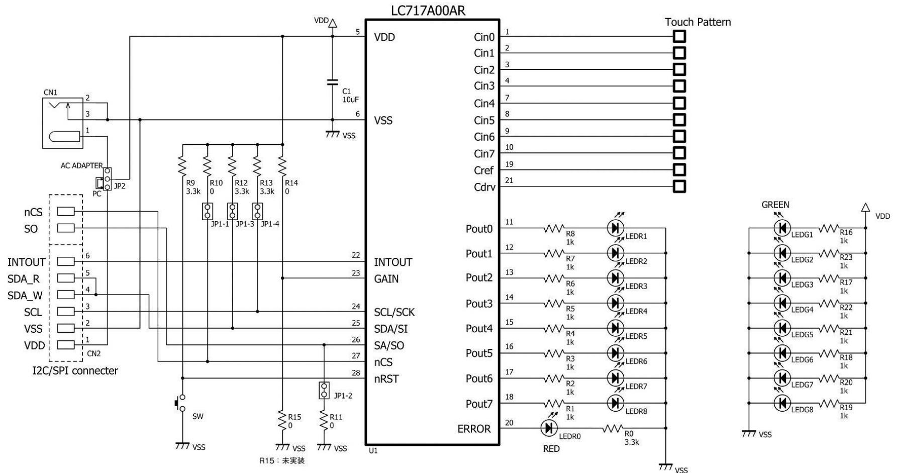
Figure 1: LC717A00AR01GEVB
