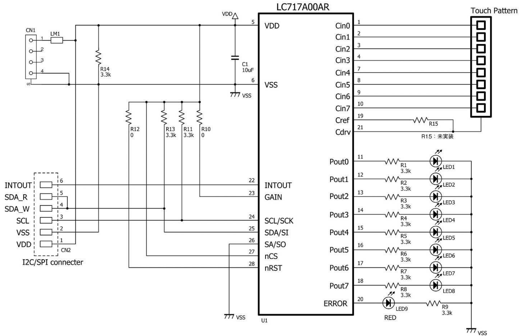
Figure 3: LC717A00AR03GEVB
